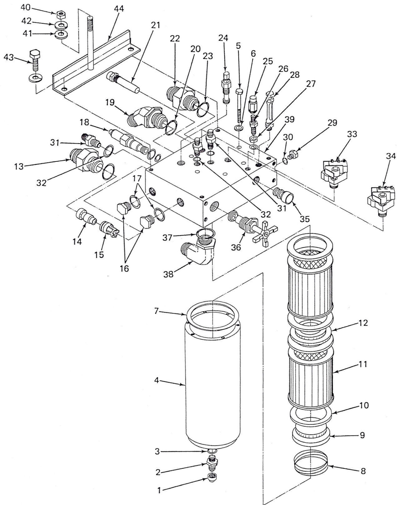
Figure 9. Low Pressure Manifold Assembly
