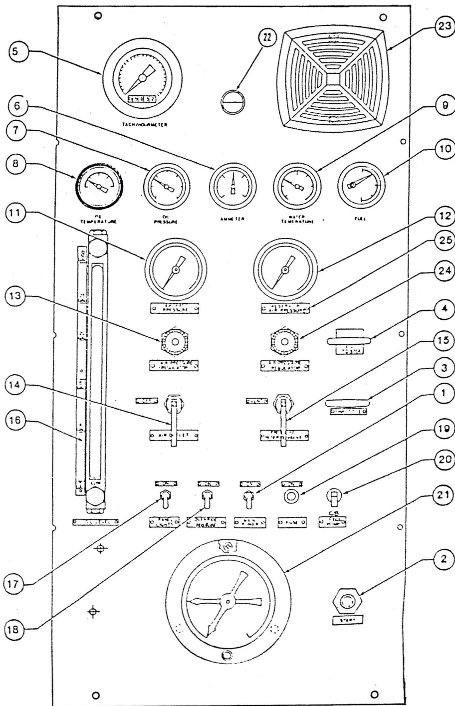
Figure 17. Auxiliary Panel Controls and Instruments (Sheet 1 of 2)
