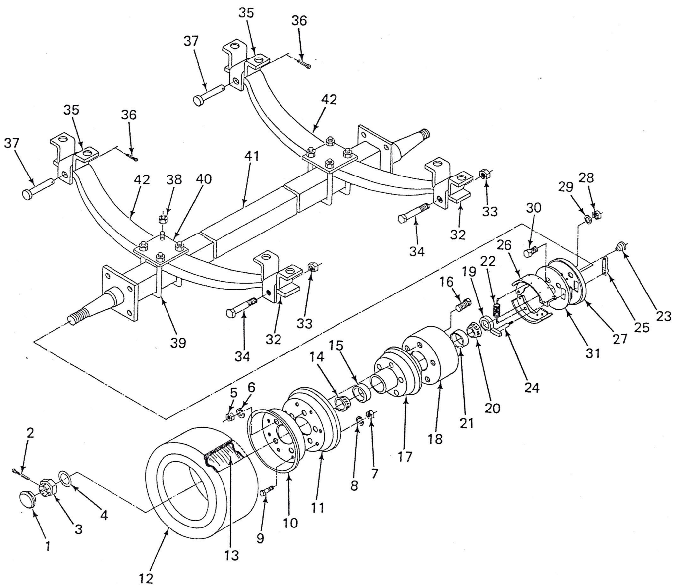
Figure 29. Rear Axle Assembly
