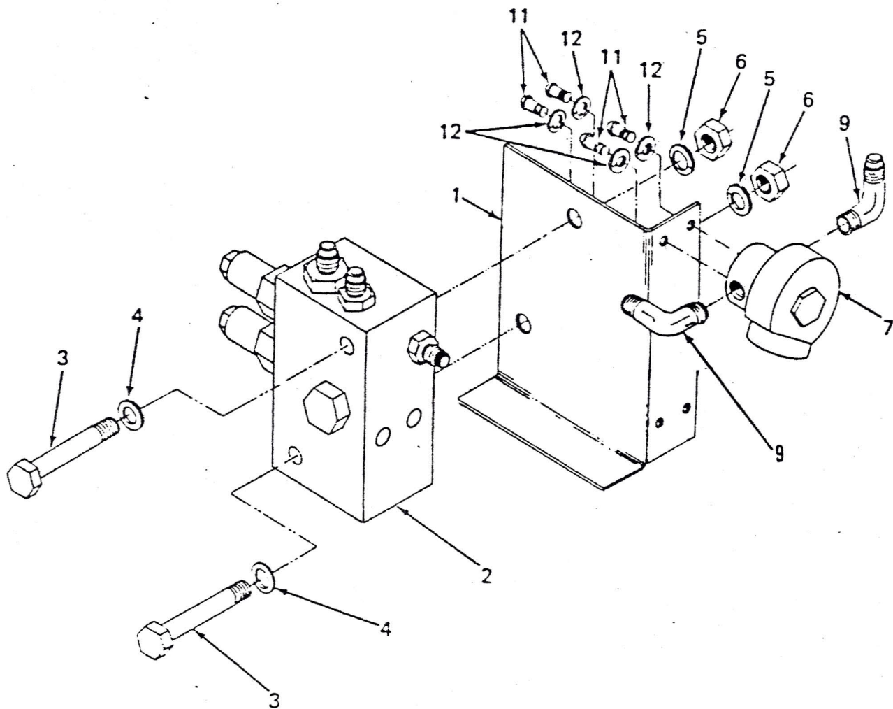
Figure 4. Fill Manifold/Solenoid Valve Assembly
