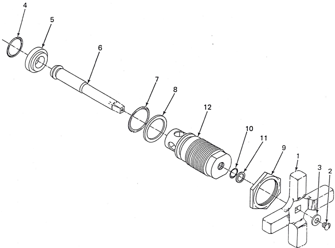
Figure 13. Throttling Valve Assembly
