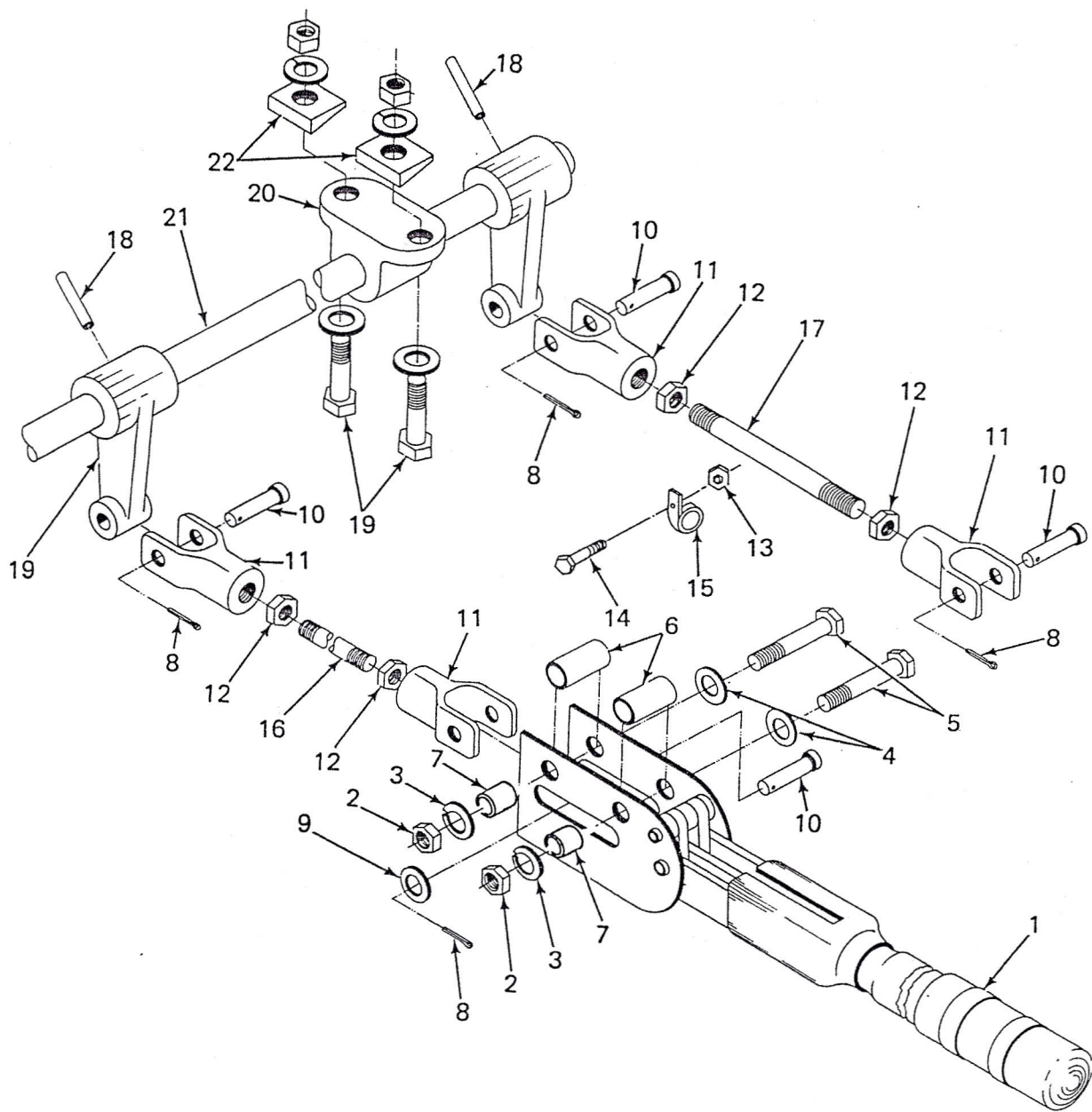
Figure 28 Handbrake Lever and Cross-Shaft Assembly
