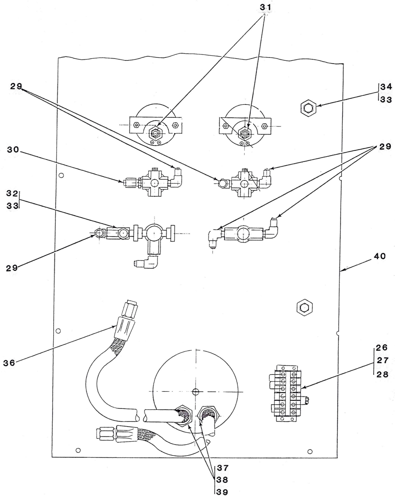
Figure 17. Auxiliary Panel Assembly (Sheet 2 of 2)
