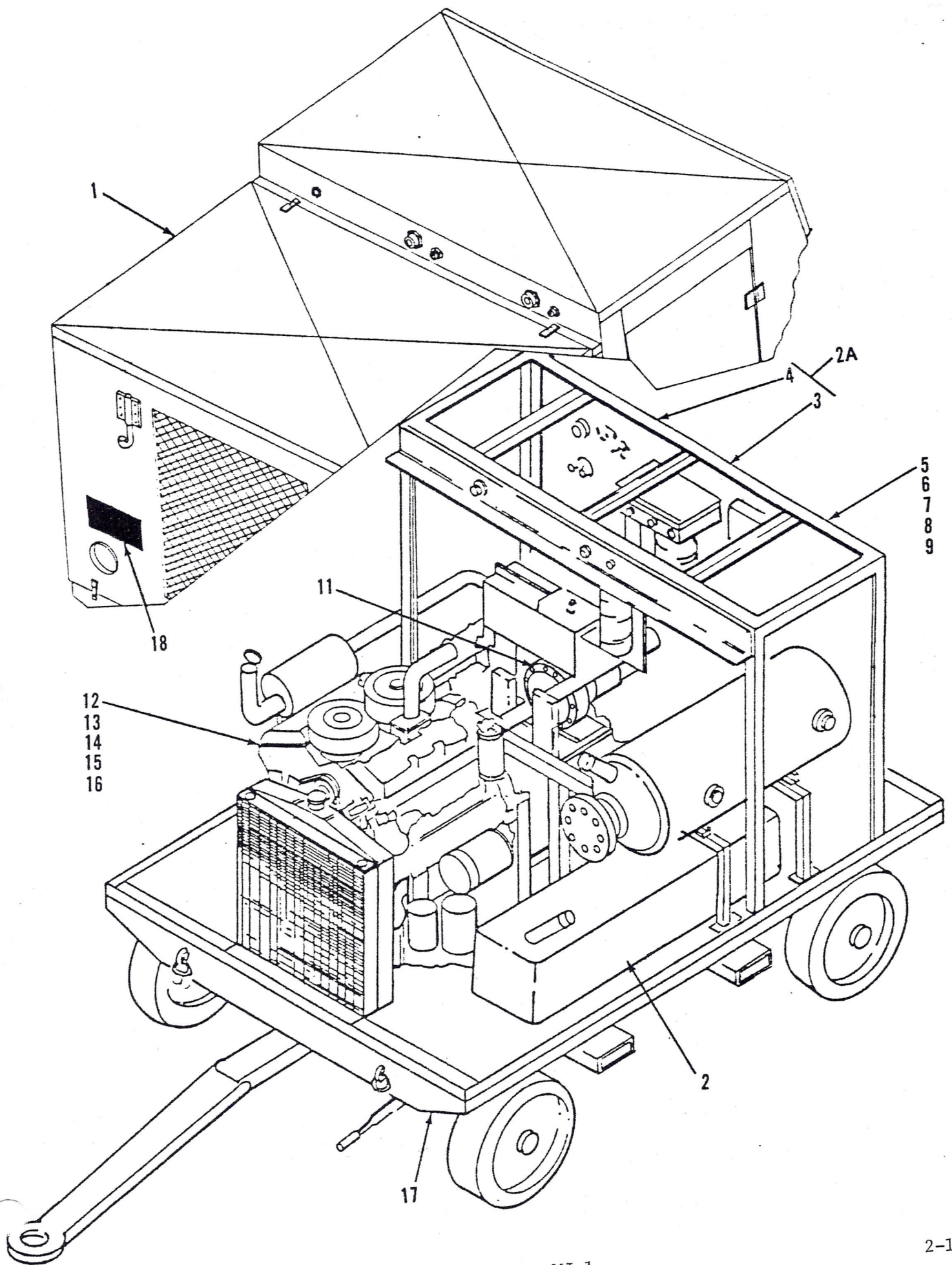
Figure 1. Major Components, MJ-1
