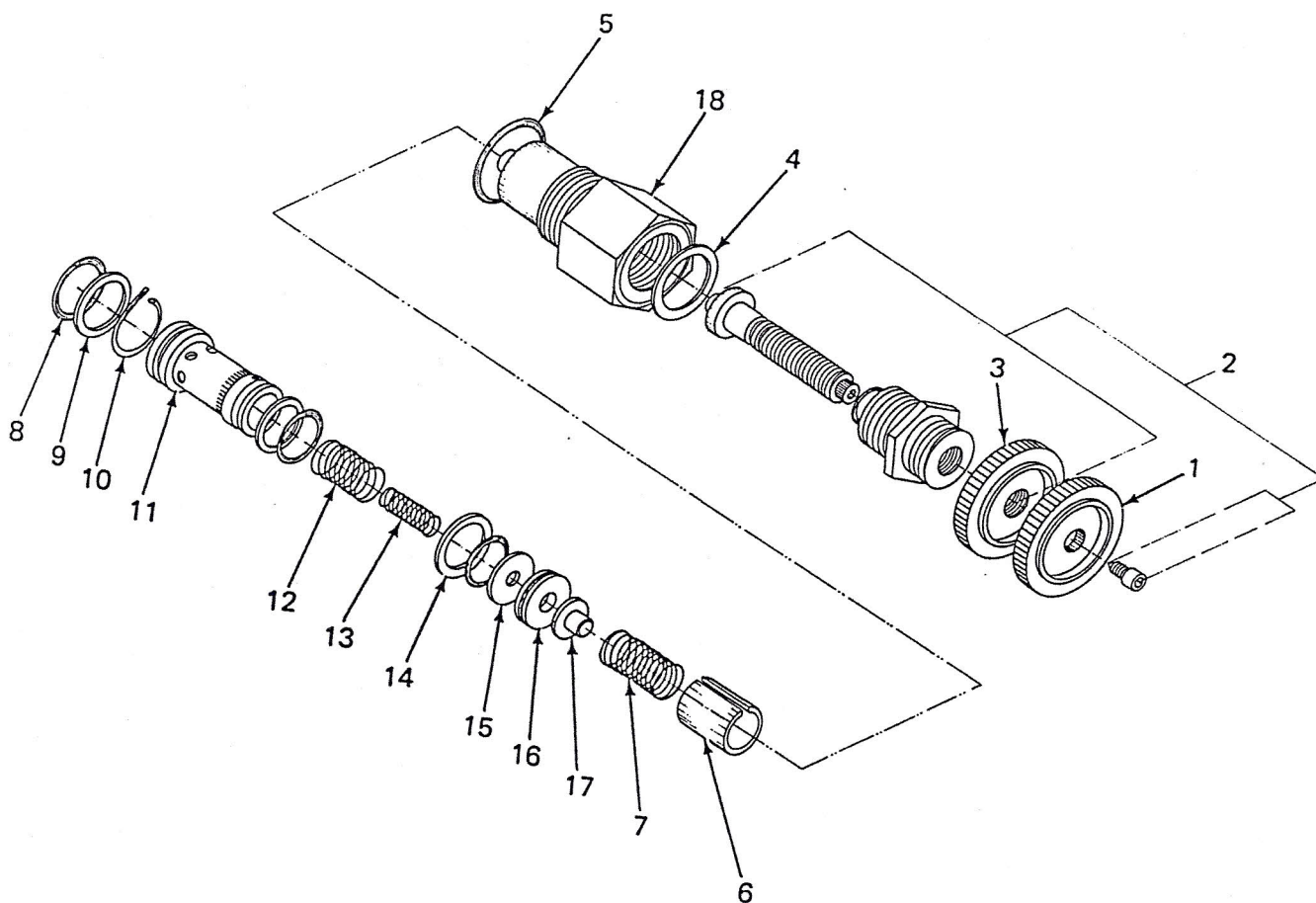
Figure 16. High Pressure Relief Valve
