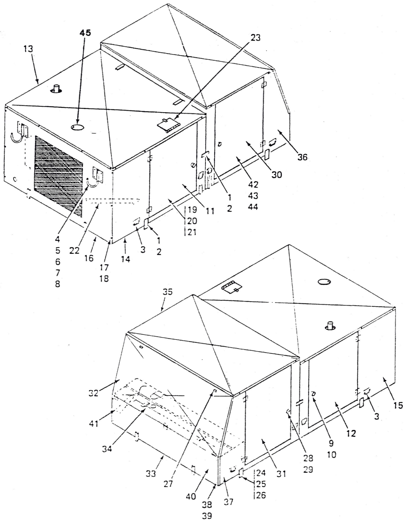
Figure 2. Housing Assembly
