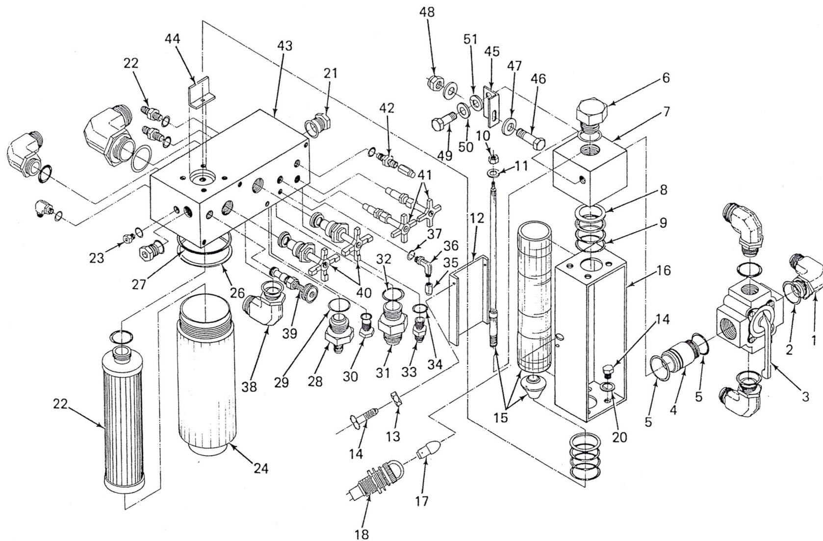
Figure 14 High Pressure Manifold Assembly
