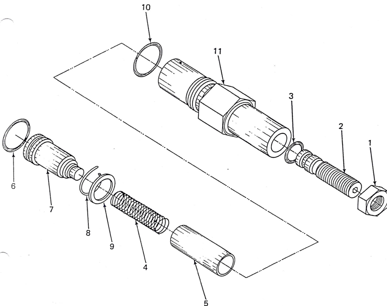
Figure 6. Low Pressure Relief Valve
