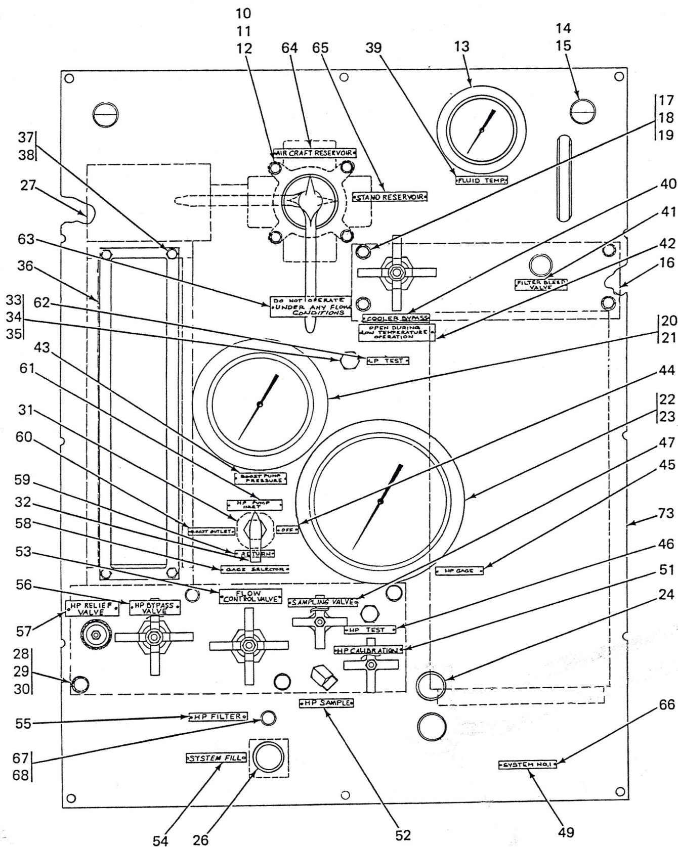
Figure 8. Hydraulic Panel Assembly (Sheet 1 of 2)
