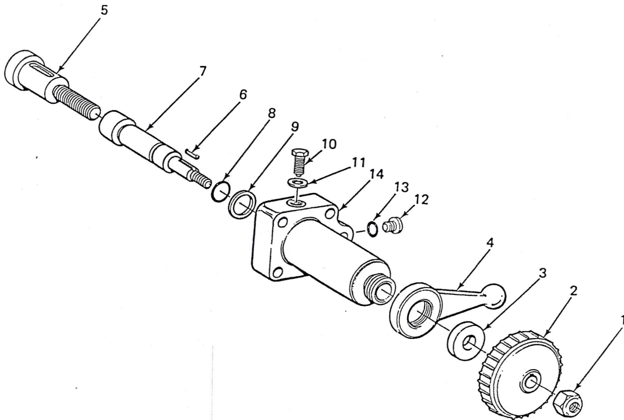
Figure 22. Displacement Control Assembly
