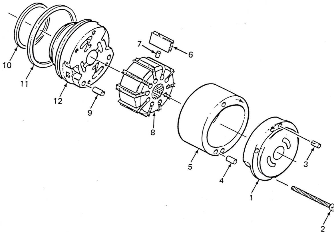
Figure 24. Boost Pump Cartridge Assembly
